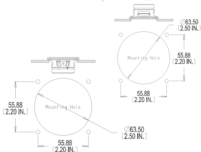
Figure 1 - Face Mounting (Recommended)
