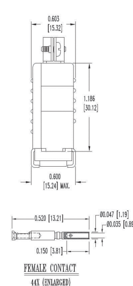
D-sub Connector, 44 pin
