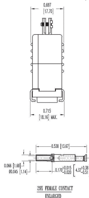
D-sub Connector, 29 pin
