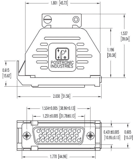
Positronic RD29S10JVLX
