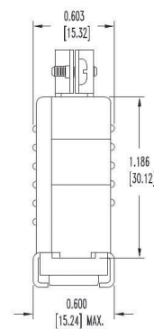
D-sub Connector, 44 pin
