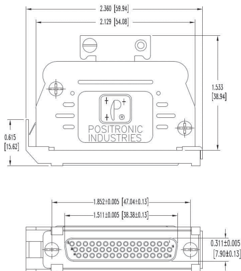
Positronic DD44S10JVLX
