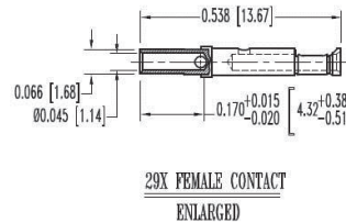
D-sub Connector, 44 pin
