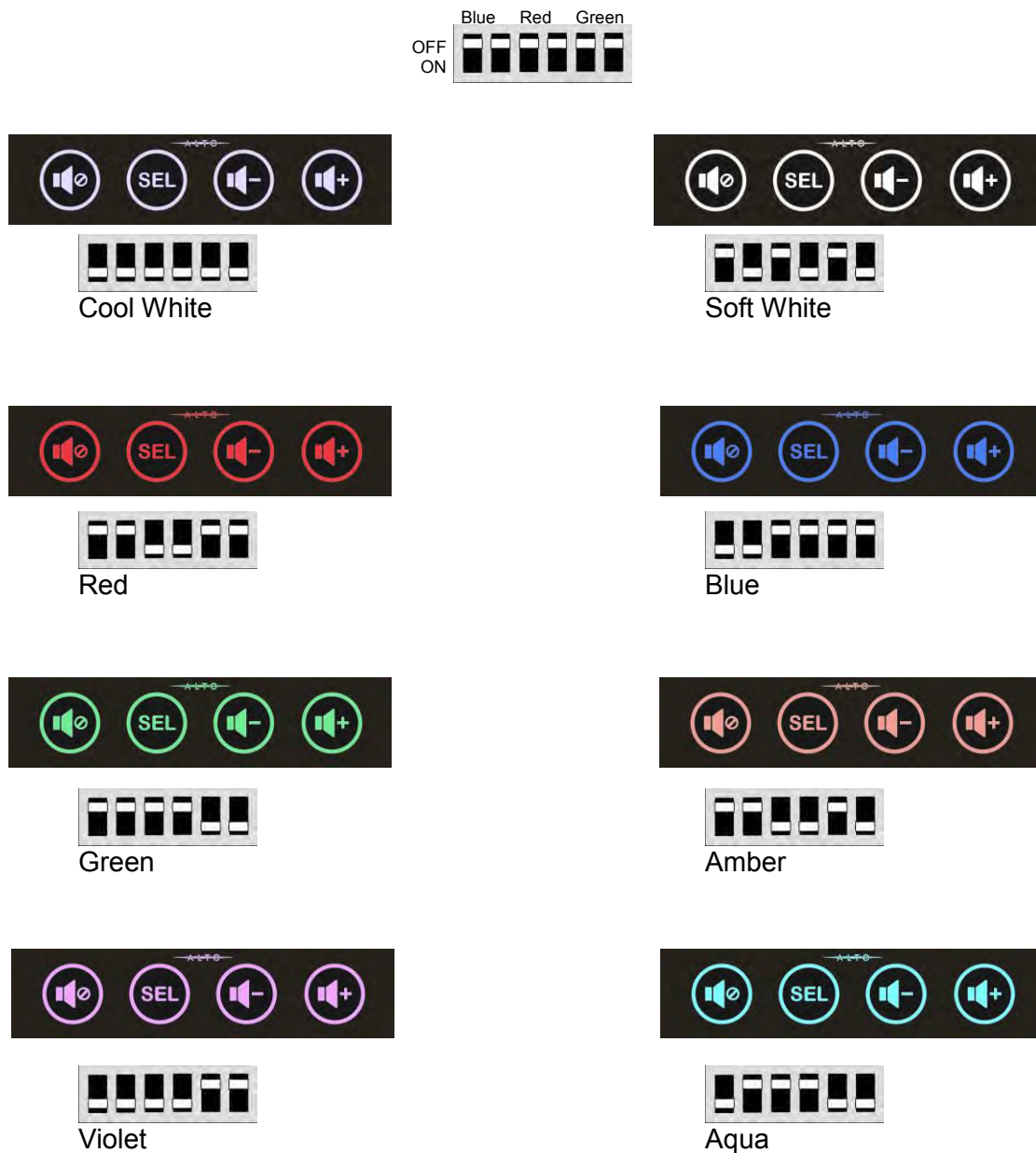
Figure 12: Example LED Color Select Diagram
