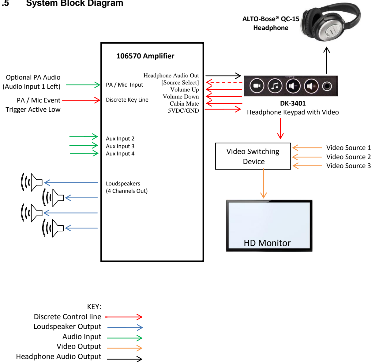
Figure 3: DK-3401 Block Diagram
