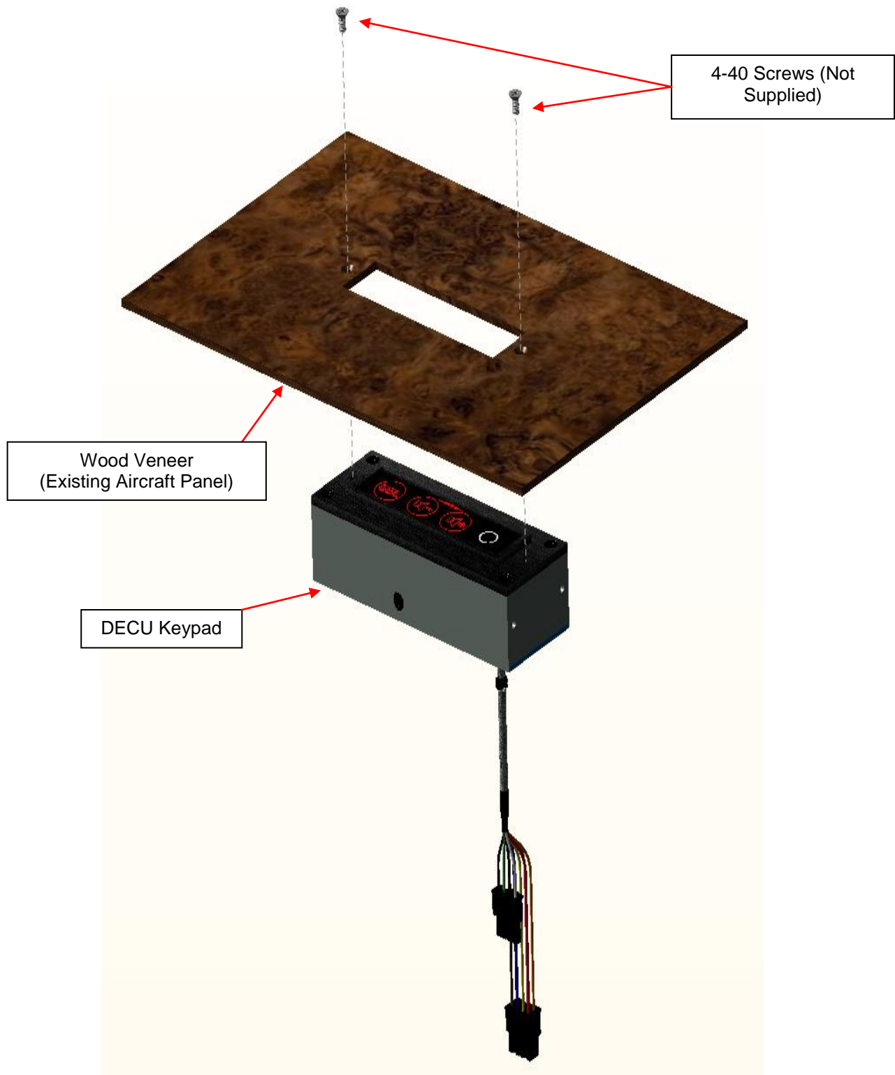
Figure 8: Keypad Thru-Panel Mounting
